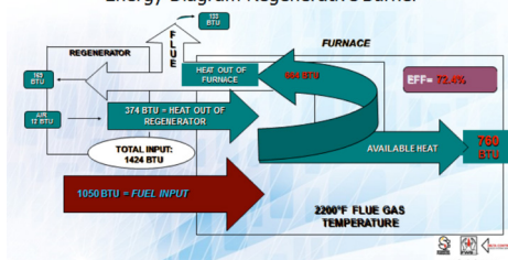
Energy Diagram Regenerative Burner
