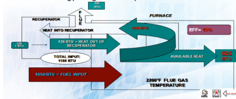
Energy Diagram Recuperative Burner
